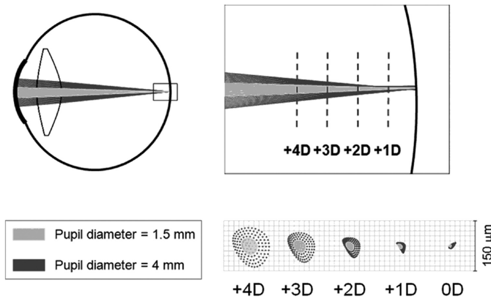
FIGURE 1. Exact ray tracing is performed in an eye model with two different pupil sizes, 4-mm diameter ( dark rays ) and 1.5-mm diameter ( lighter rays ). The area close to the retina is zoomed in for a better observation of the increase in depth of focus. The impact of rays (for both pupil sizes) at different planes separated by a 1 D distance from the retina are shown in the lower right .
