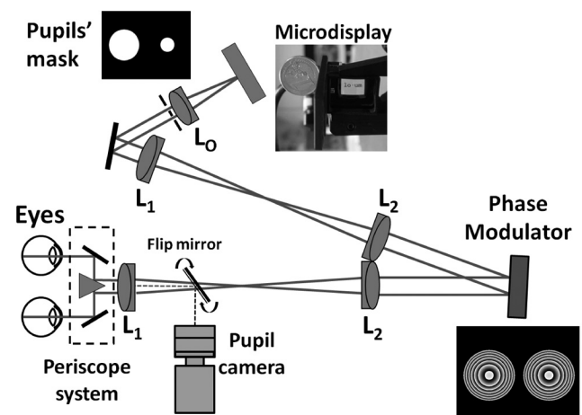
FIGURE 2. Experimental setup for binocular visual simulation. Defocus was generated by the phase modulator. Asymmetric entrance pupils were combined under different luminance conditions in monocular and binocular vision.
